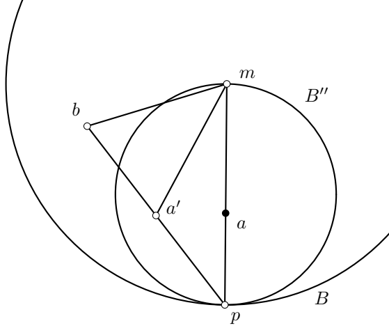
Figure 4: Proving that b \in B .
