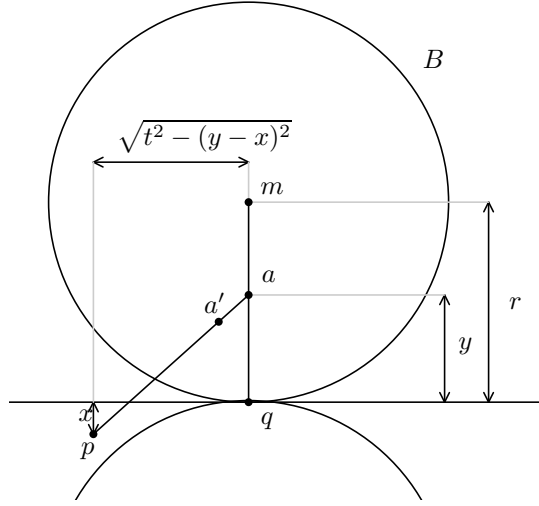
Figure 2: t' is again a violator.
