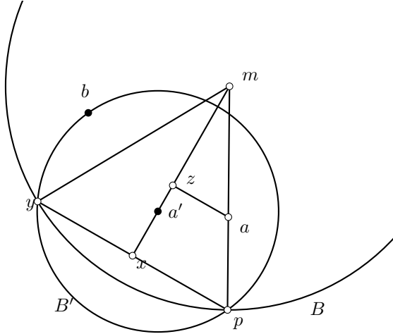
Figure 3: Estimating the diameter of B' \setminus \text{int } B .
