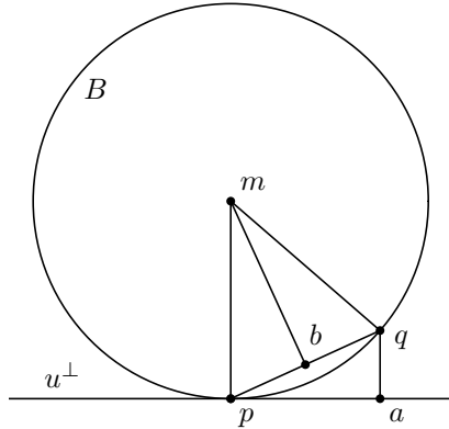
Figure 1: The component of q - p in any normal direction is small.
